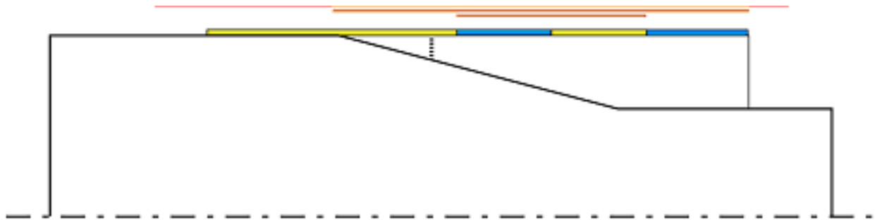
Figure 8. The diagram shows, schematically, the position of the breakdown relative to the first bifurcation in the stator windings. Again, the diagram is taken from the above SAIC internal report.
