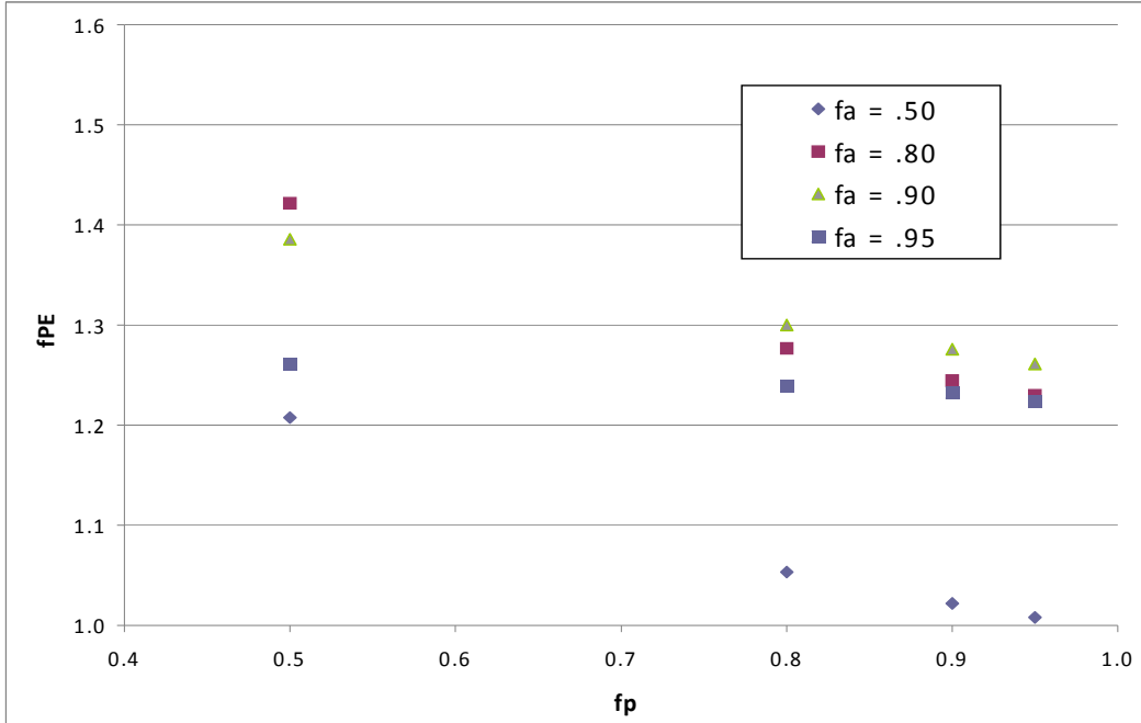
Figure 24. Shows the enhancement factor for a fixed value of the parameter fw=0.05 . The abscissa is the packing fraction, fp. The four individual curves are for different values of fa.
