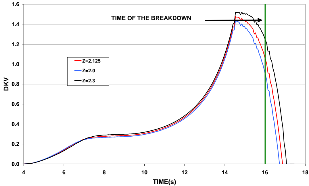
Figure 14. Showing the variation in voltage drop realized by monitoring different positions in the HFCG.
